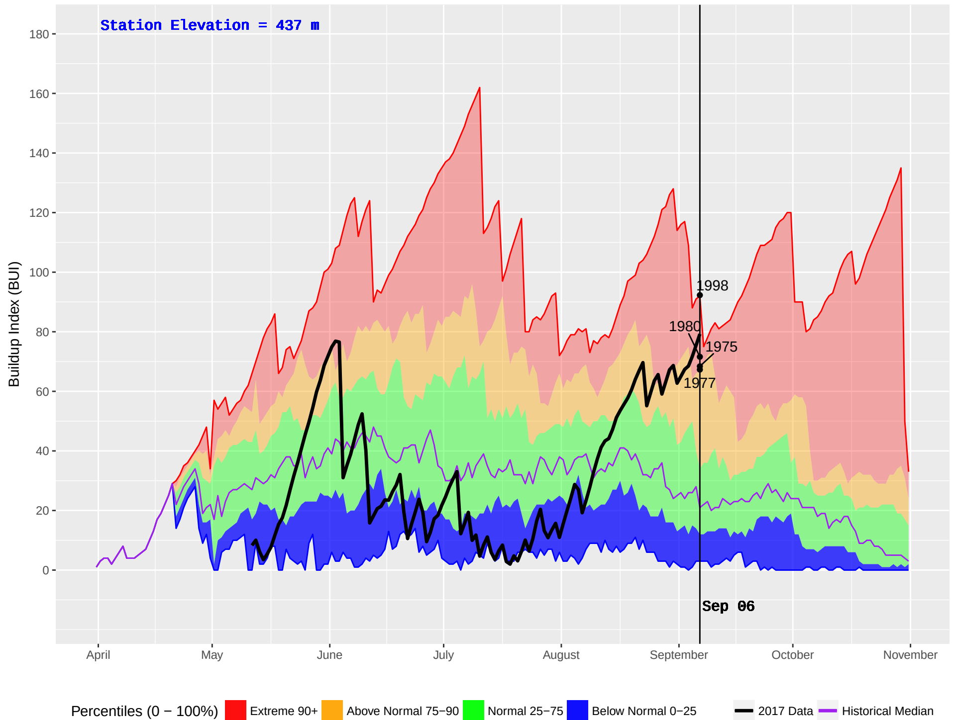
ELK MOUNTAIN (438) : Historical (1973–2016) and Current (2017) Noon Buildup Index (BUI)
